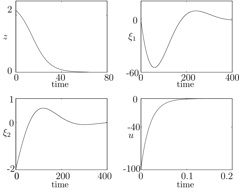
Figure 4.8: Linear high-low gain design (4.5.36): fast peaking of u and slow peaking of \xi_1 .
